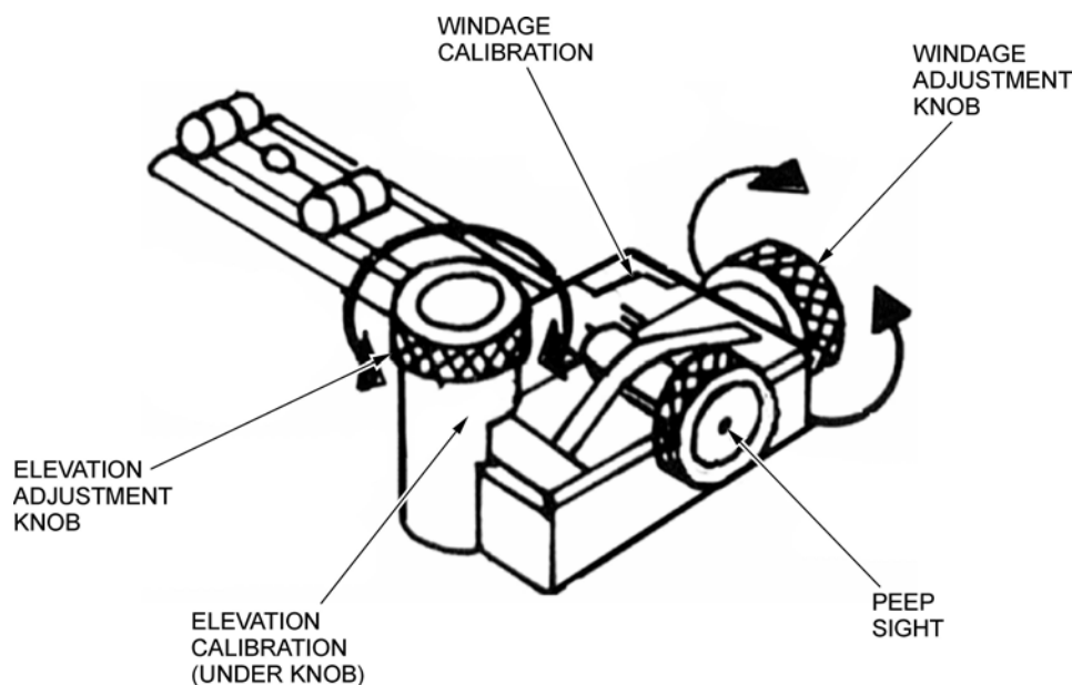
Figure 6-3-3 Sight Adjustment of the Cadet Air Rifle
