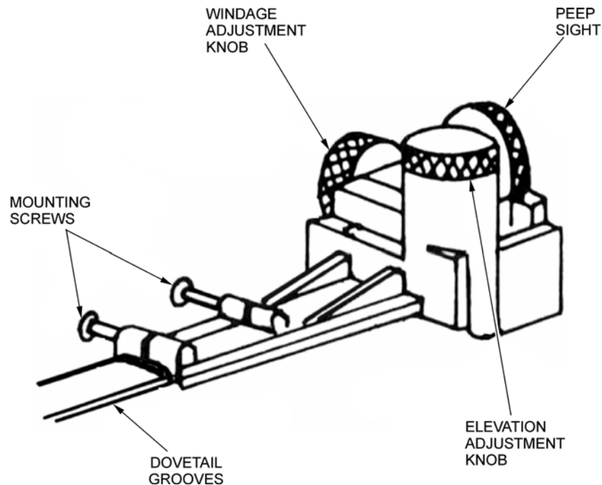
Figure 6-3-2 Rear Sight of the Cadet Air Rifle
